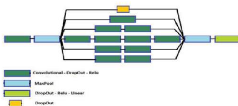
Fig. 4.2 Network architecture
